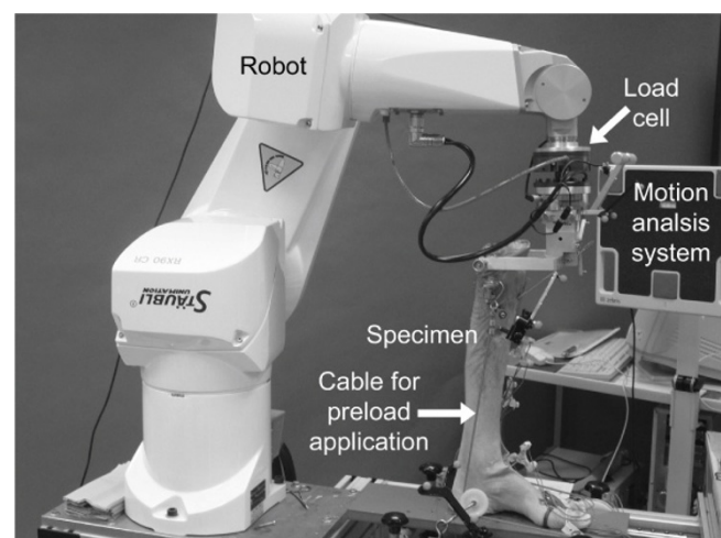
Figure 1 Setting with robot, specimen, and motion analysis system. Specimen mounted to the robot and footplate and equipped with ultrasound transducers.
